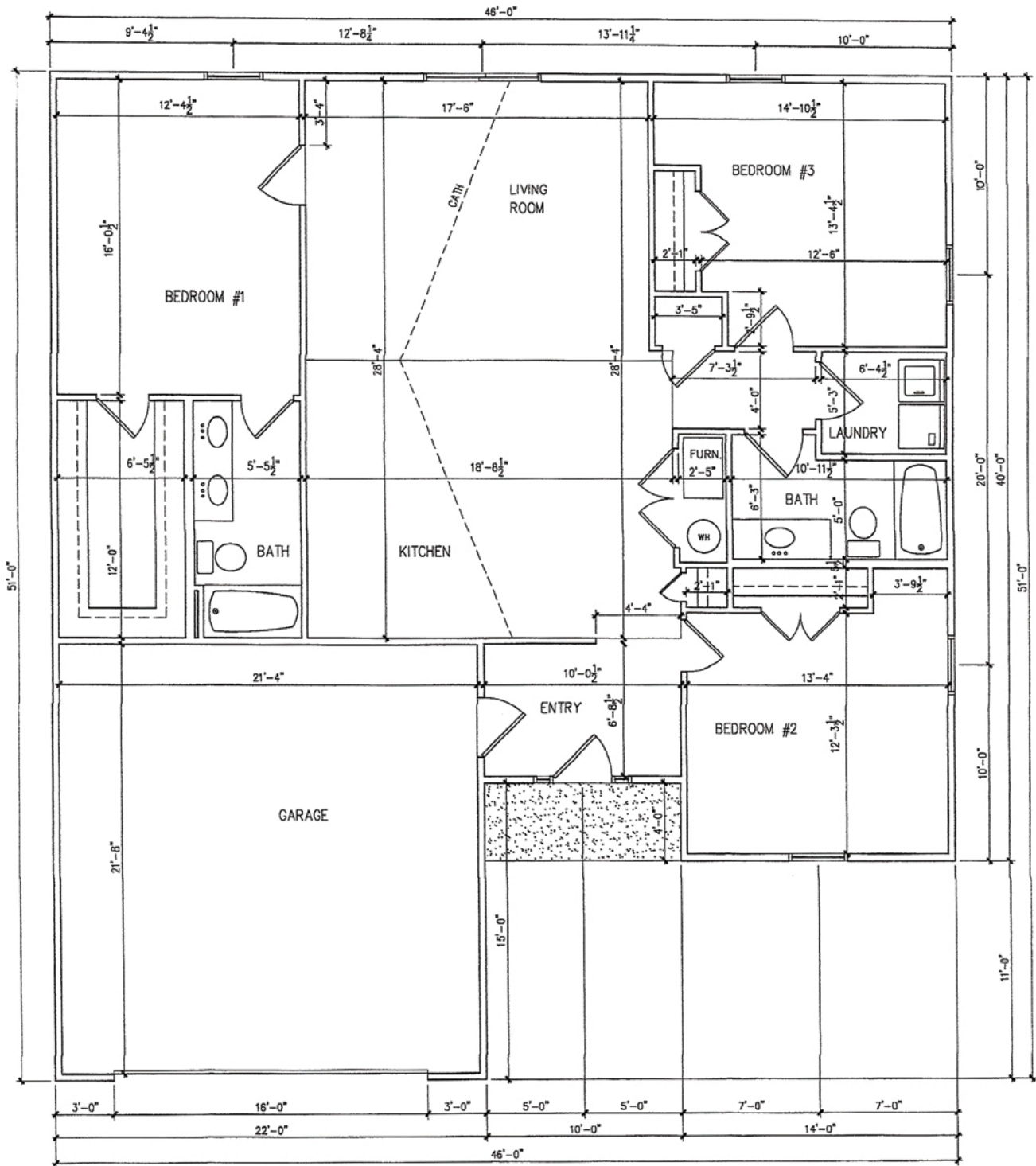
FLOOR PLAN - C 1/4" = 1'- 0"
