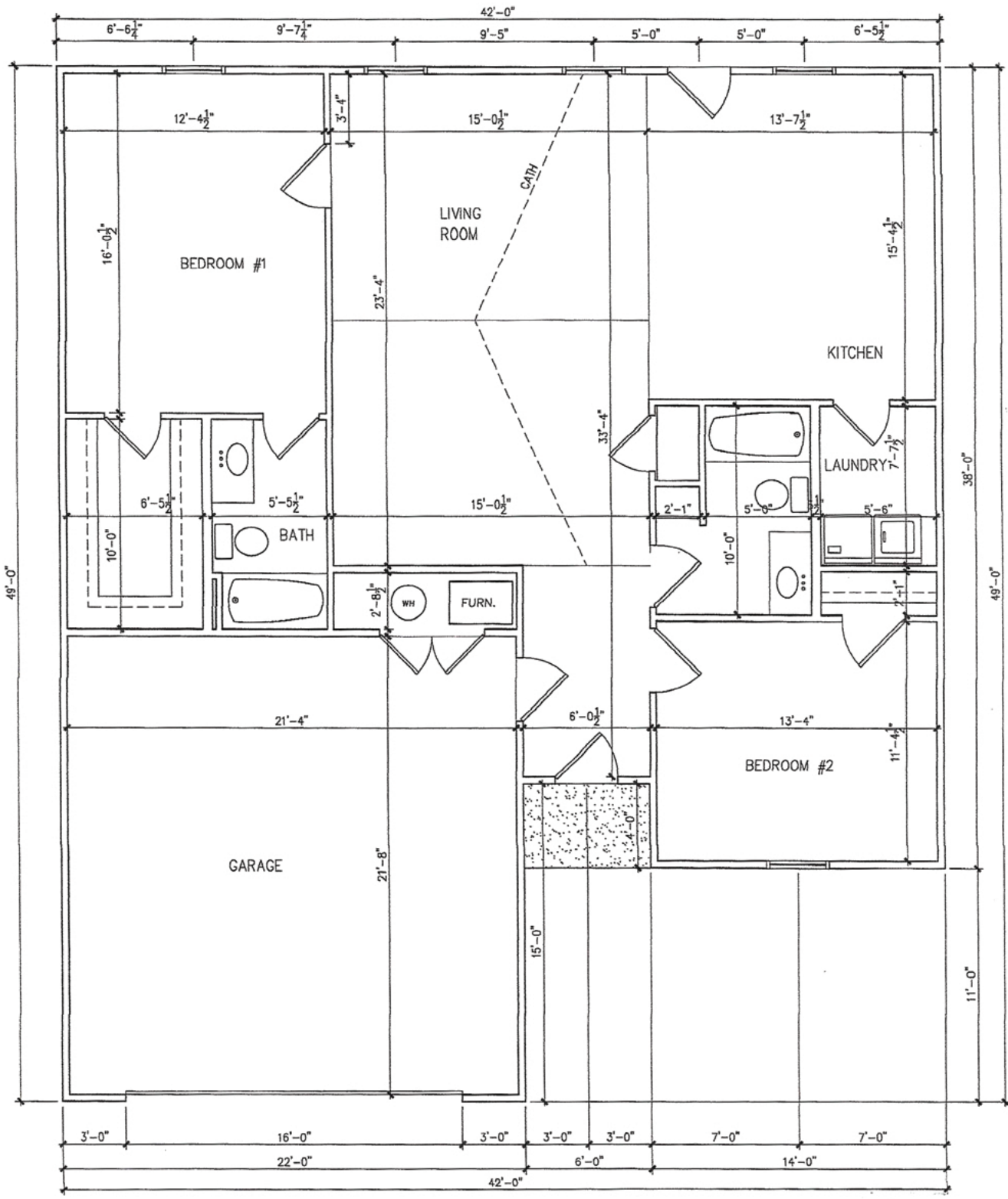
FLOOR PLAN - B 1/4" = 1'- 0"
