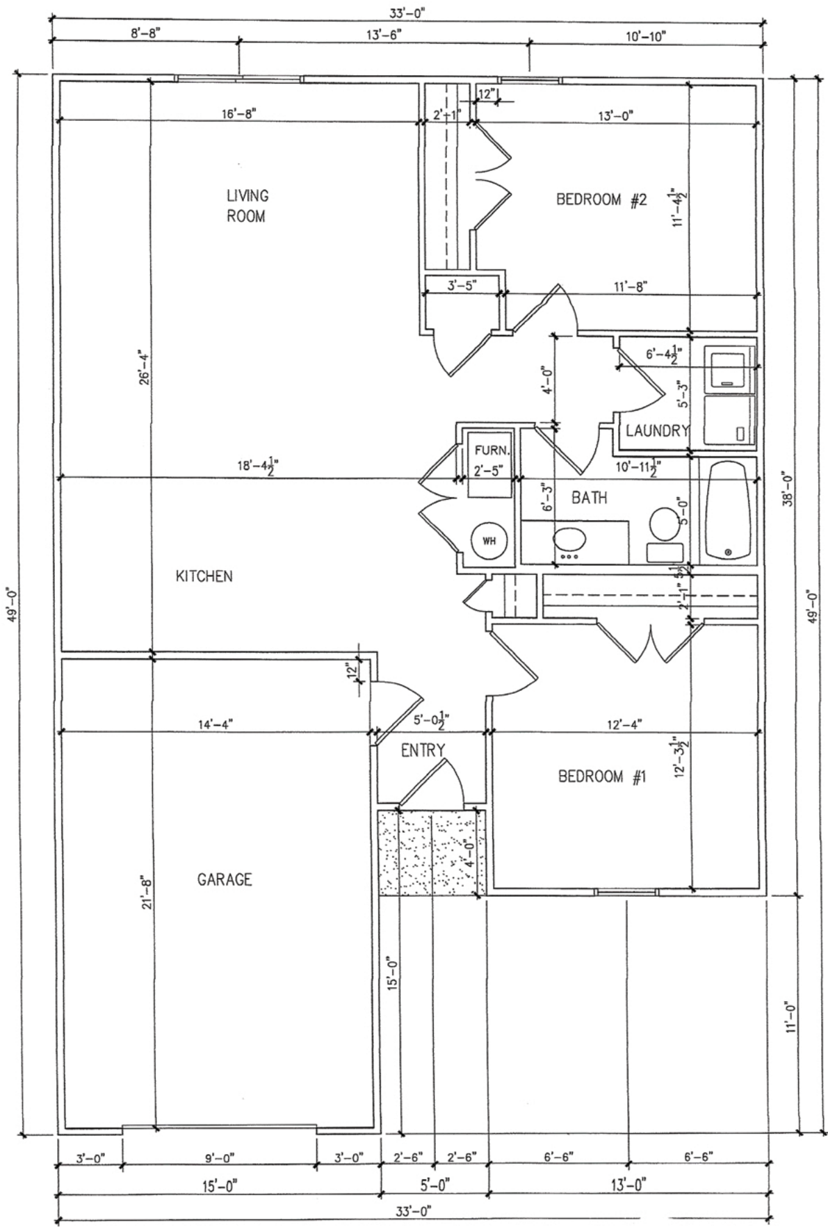
FLOOR PLAN - A 1/4" = 1'-0"
